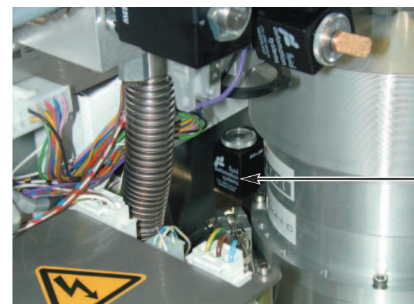
LDS valve (connected to the TMP 5154 rear)
