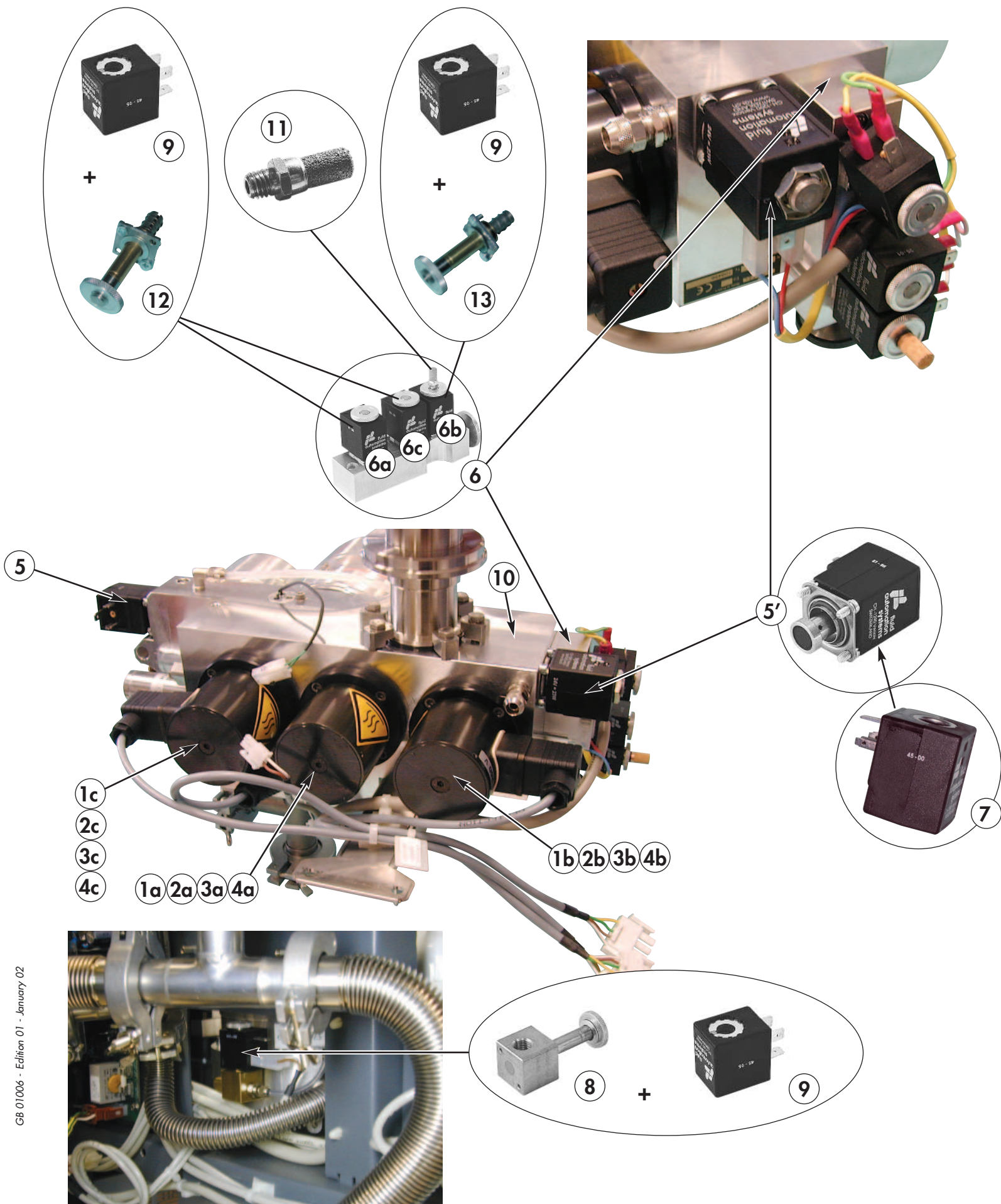
LDS valve (connected to the TMP 5154 rear)
