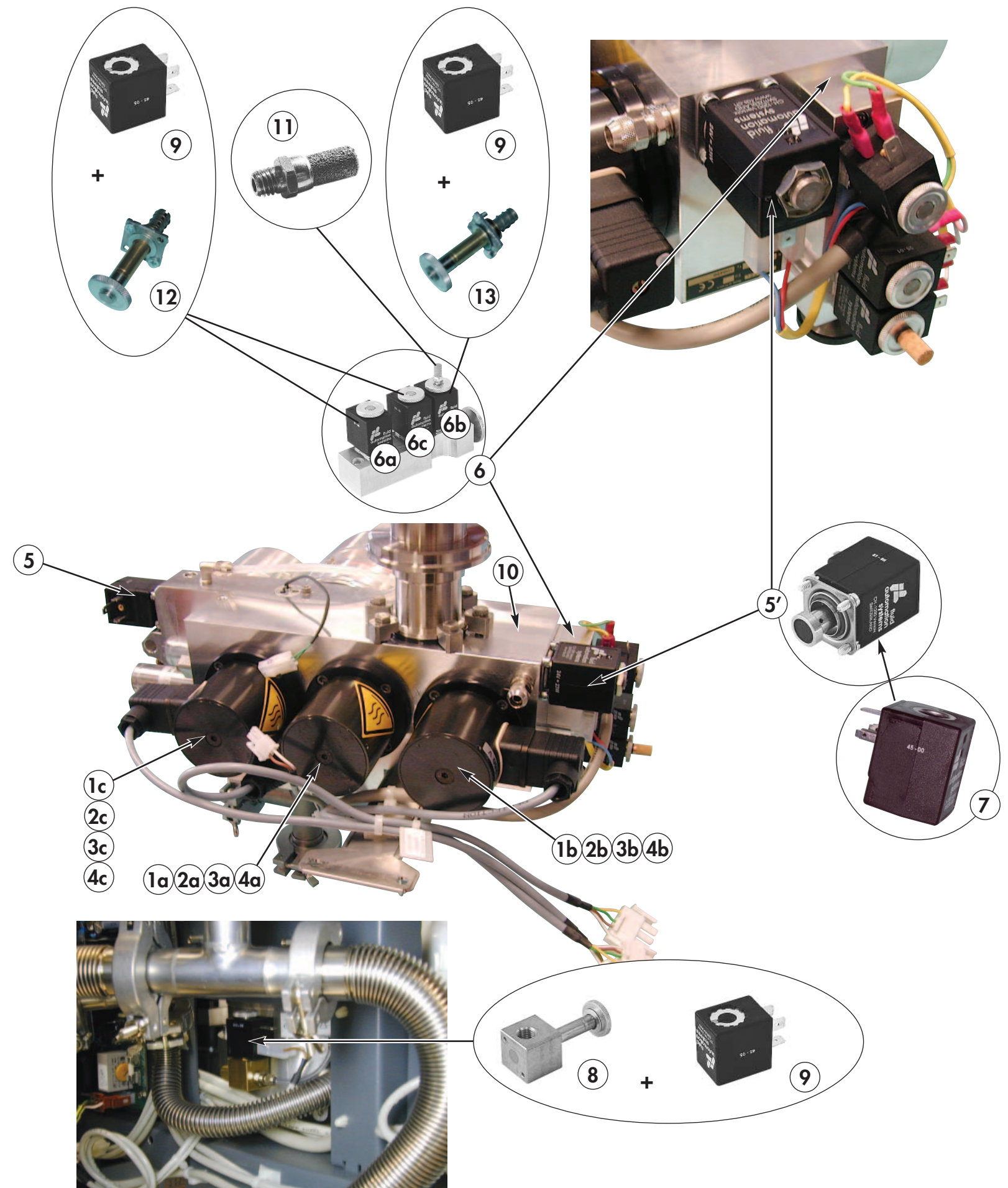
LDS valve (connected to the TMP 5154 rear)
