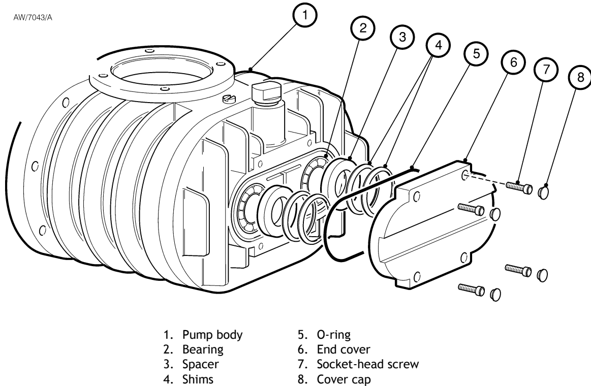
Figure 10 - Lubricate the rear bearing (EH250FX, EH500 and EH500FX pumps only)
