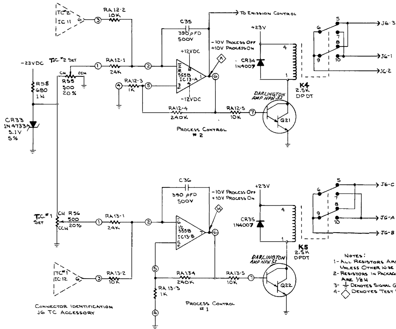
FIG.5-9 THERMOCOUPLE PROCESS CONTROL SCHEMATIC
