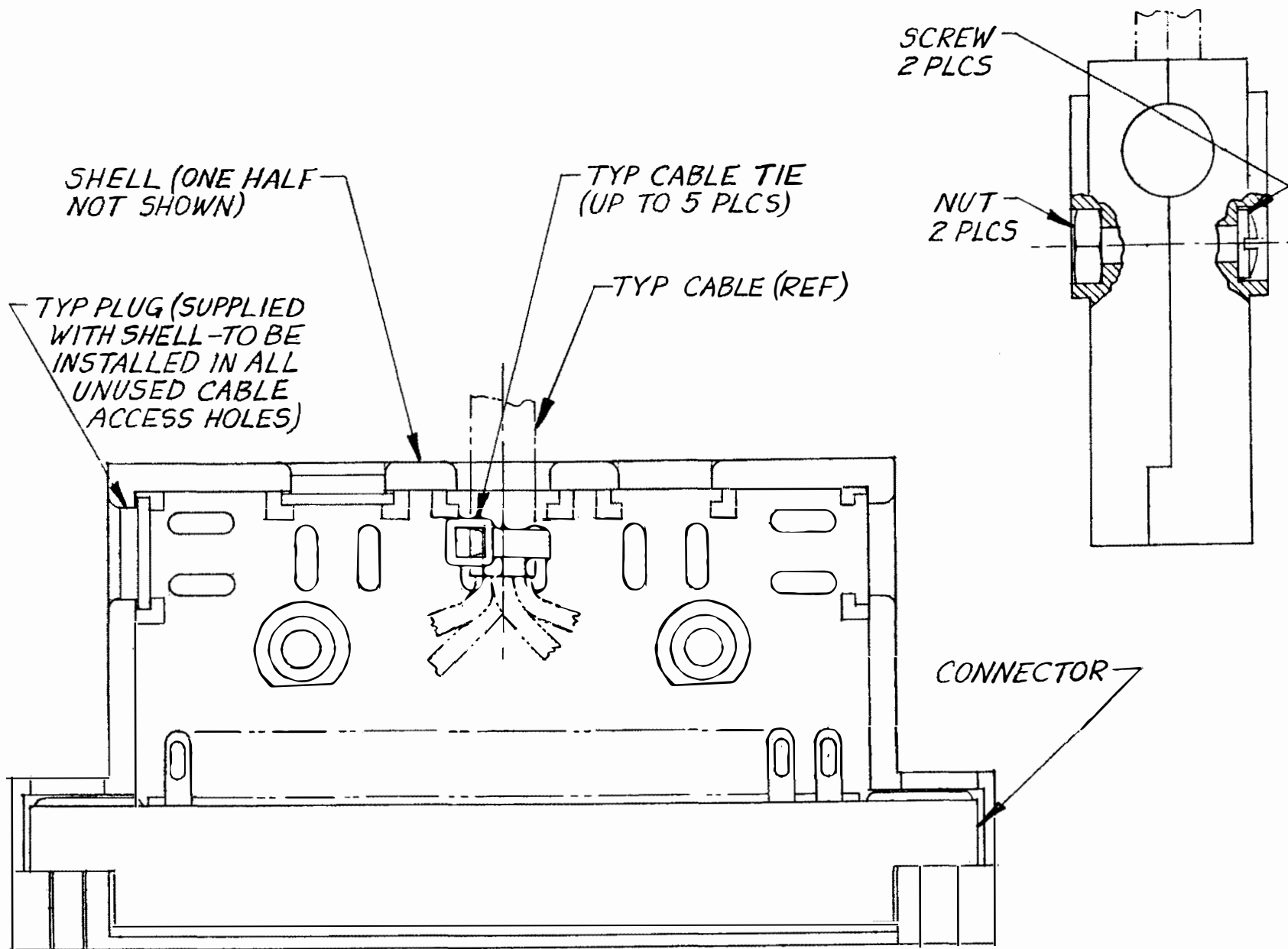
FIG. 3-3A CONNECTOR PICTORIAL
