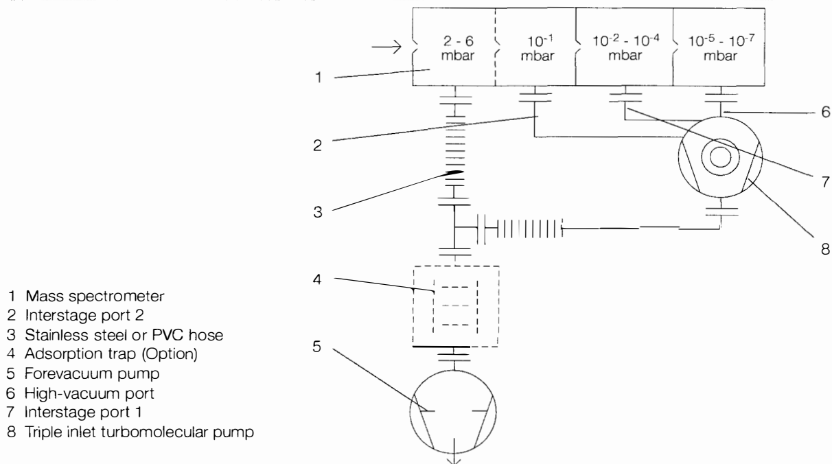
Fig. 3.5 Schematic of a triple inlet turbomolecular pump system
