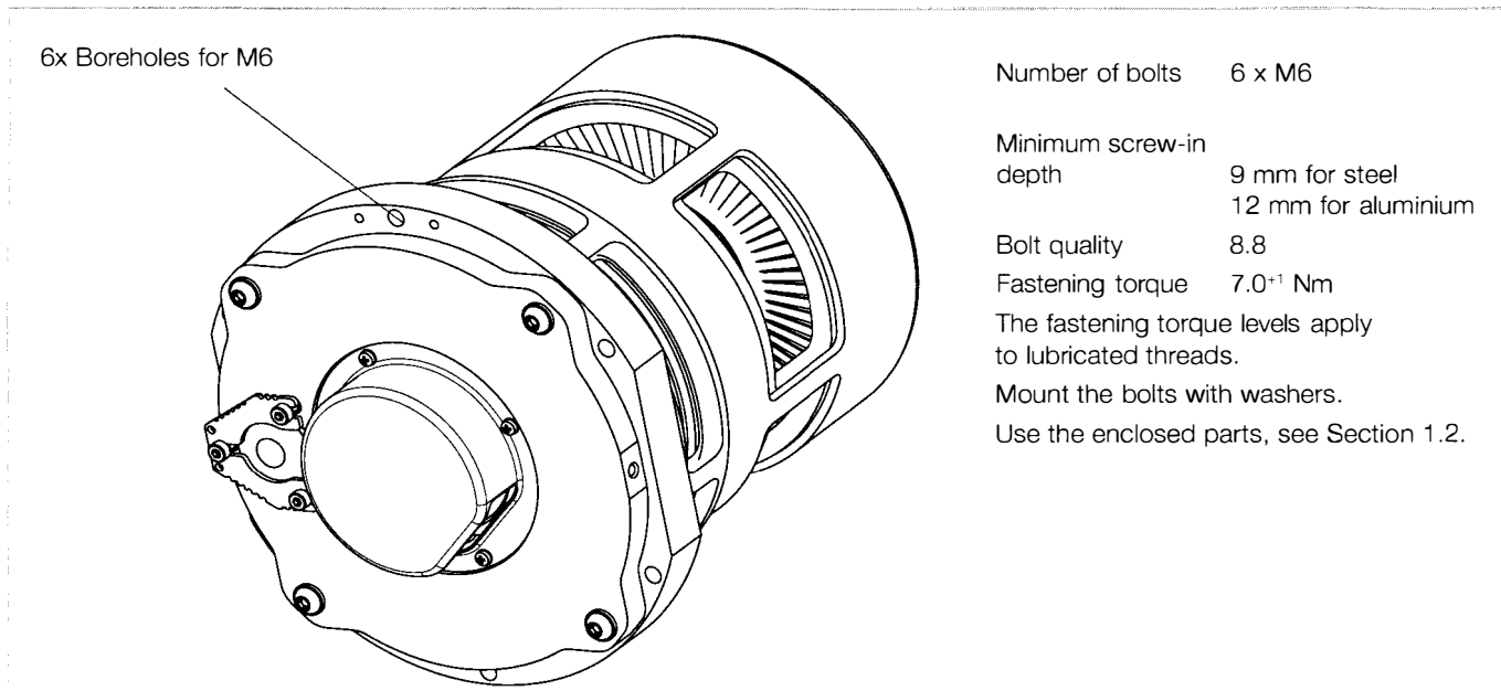
Fig. 3.2 Mounting the pump
