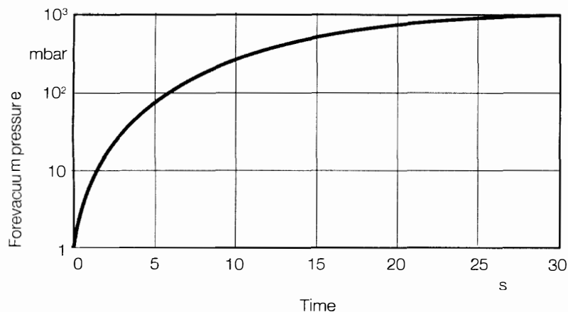
Fig. 4.2 Maximum rise in pressure
